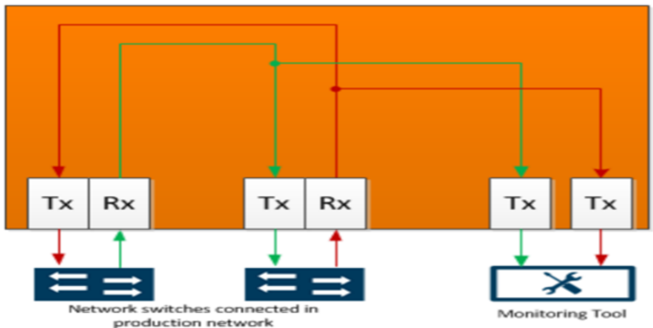
Figure 7: G-TAP A-TX21 Data Flow per Group
