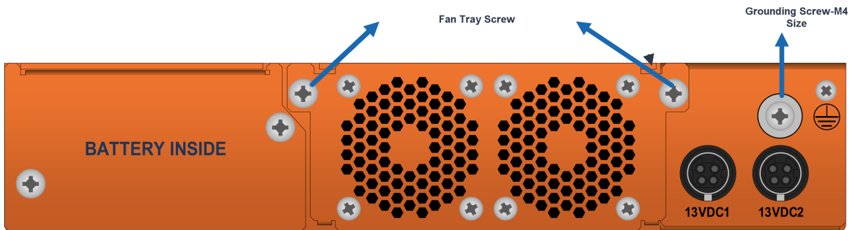
Figure 8: G-TAP A-TX21 Rear Chassis
