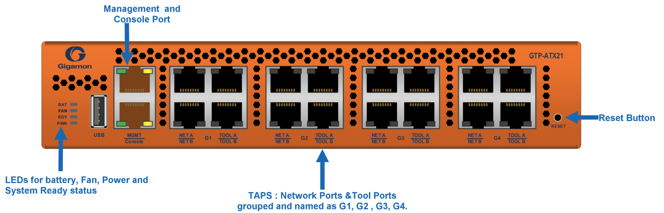
Figure 2: The G-TAP A-TX21 Front Chassis
