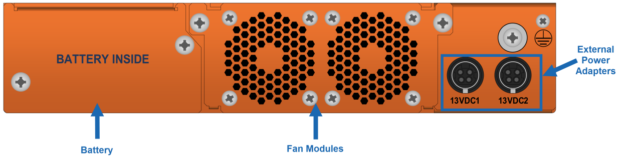
Figure 3: The G-TAP A-TX21 Rear Chassis
